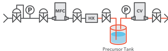
Precursor Tank
